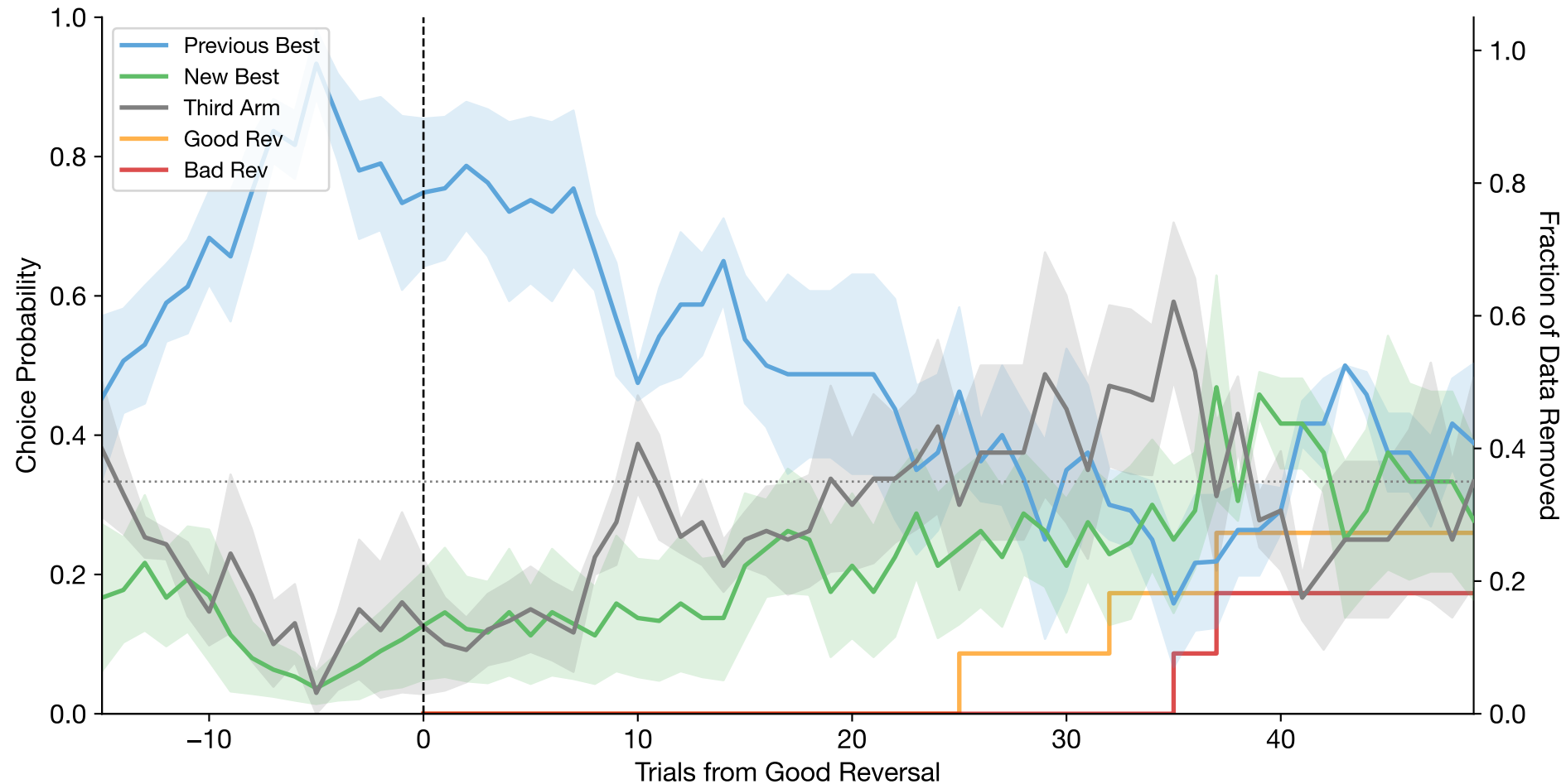
Good Reversal-Aligned Choices (mean \pm se across subjects | n=5 subjects, n=11 reversals)
